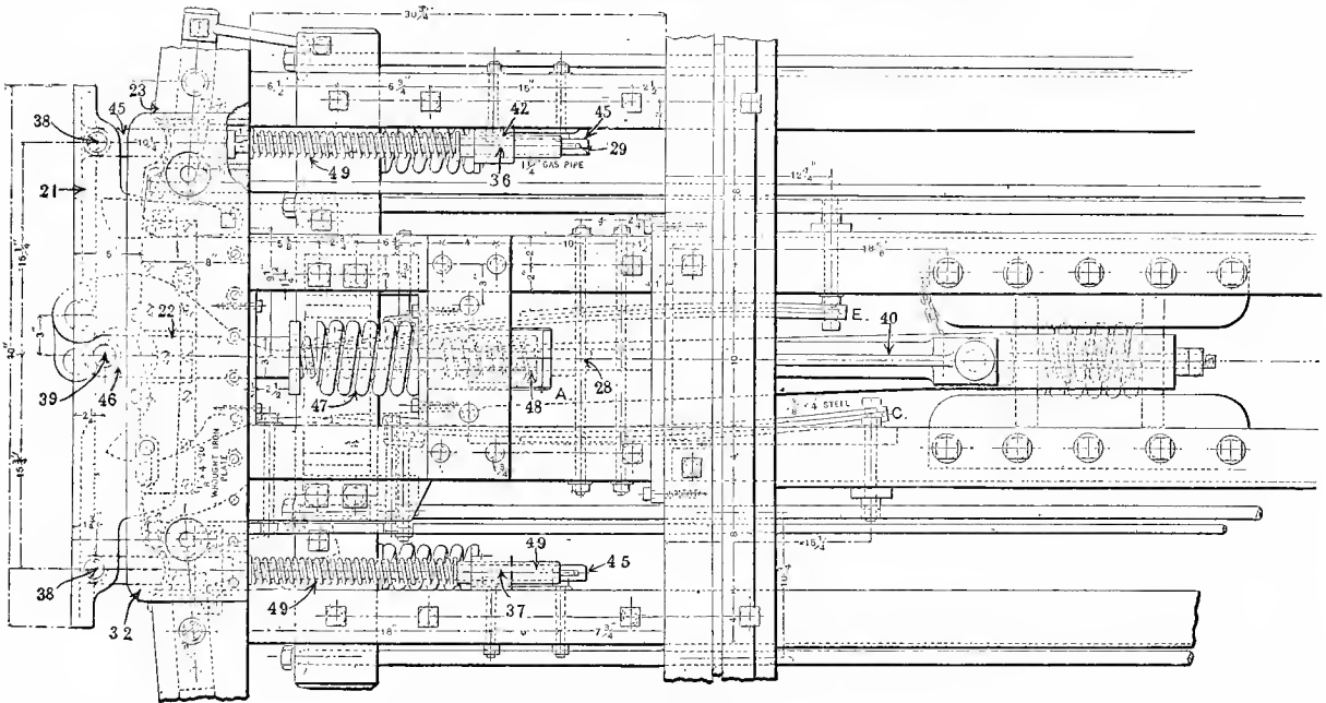
Fig. 2299. Plan of Draft Rigging.
